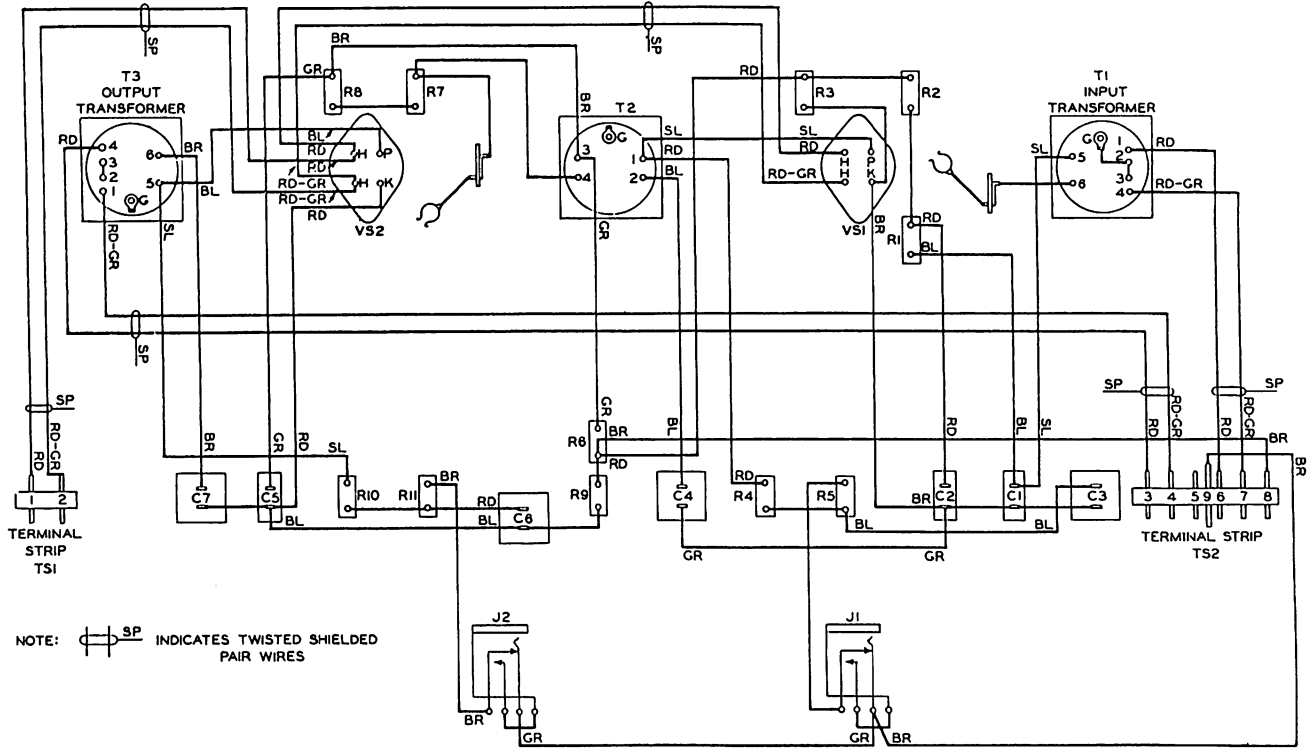
Wiring Diagram of No. 69A Amplifier
