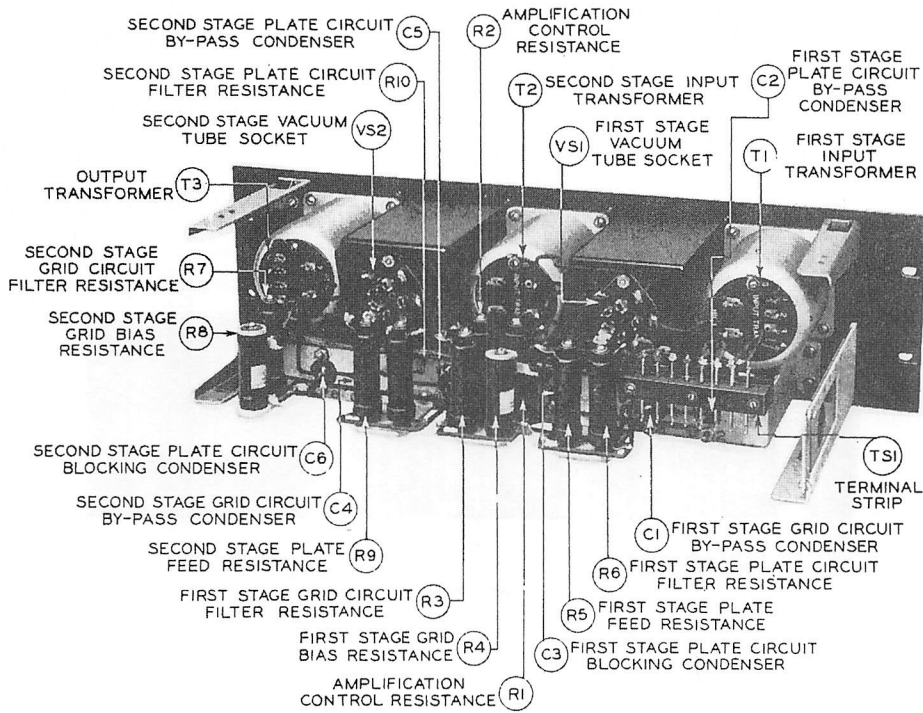
No. 61-A Amplifier—Rear View
