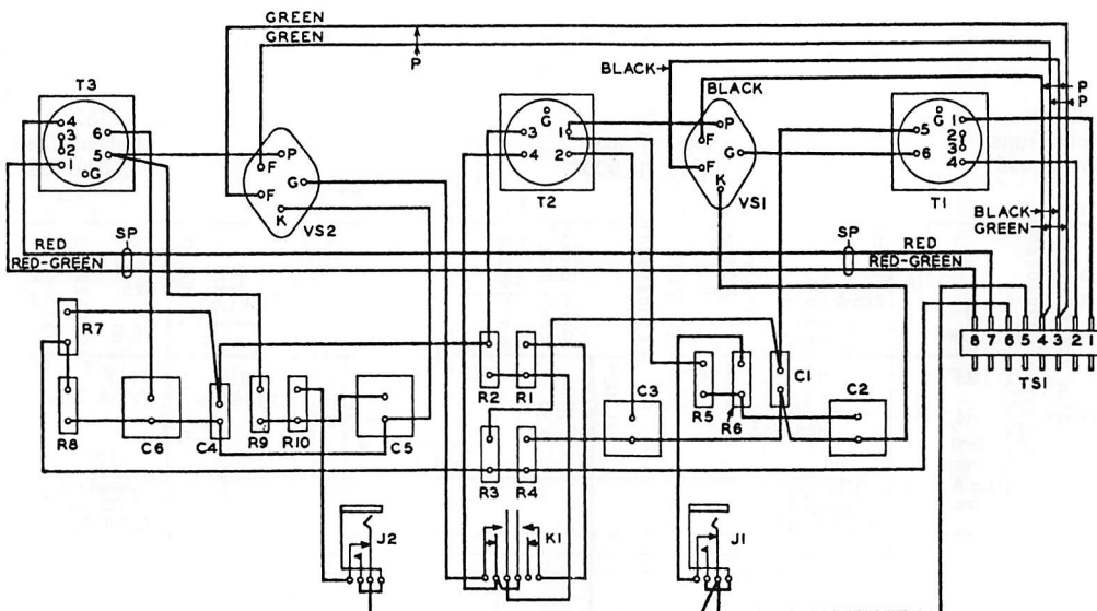
Wiring Diagram of No. 61-A Amplifier
