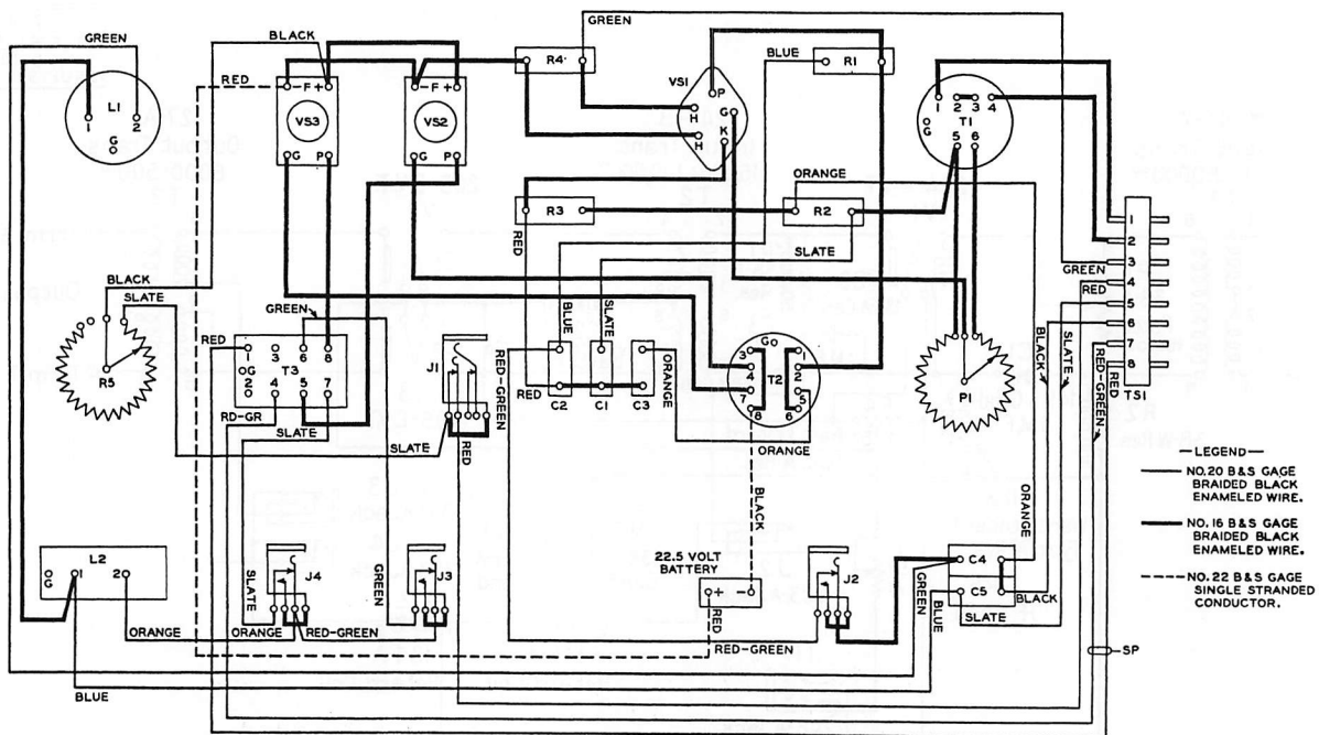
Wiring Diagram of No. 60-A Amplifier
