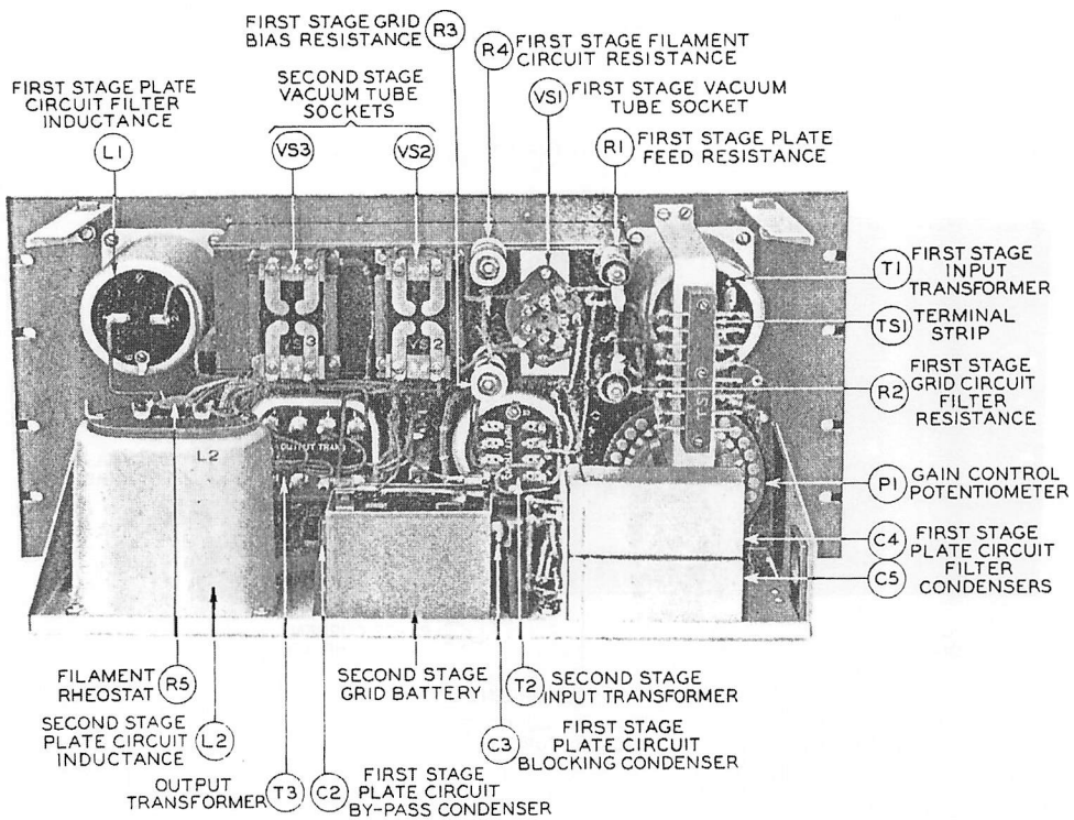
No. 60-A Amplifier—Rear View
